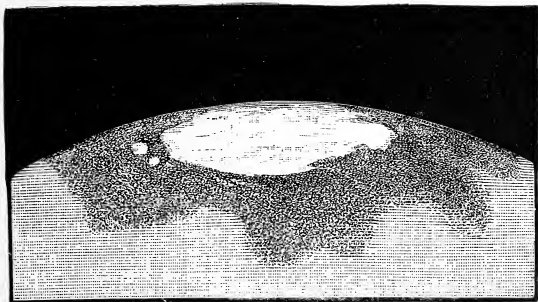
Fig. 60.—The South Pole of Mars, September, 1877. (Green.)
